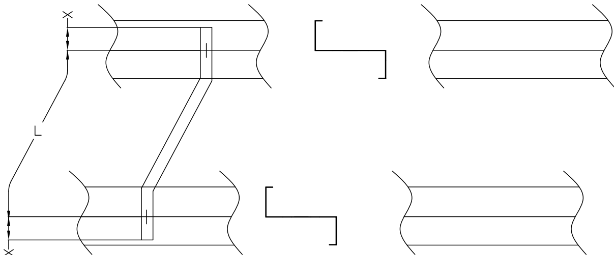
SAG RODS BRIDGING LIST SPECIFIES DIMENSION L BETWEEN PURLIN TO PURLIN DIM "X" TO BE ADDED TO THE LENGTH SPECIFIED IN BRIDGING LIST TO GET FULL LENGTH OF THE ROD
