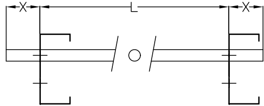
ROD BRIDGING BRIDGING LIST SPECIFIES DIMENSION L BETWEEN PURLIN TO PURLIN
