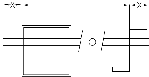
DIM "X" TO BE ADDED TO THE LENGTH SPECIFIED IN BRIDGING LIST TO GET FULL LENGTH OF THE ROD
