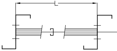
STANDARD BRIDGING BRIDGING LIST SPECIFIES DIMENSION L BETWEEN PURLIN TO PURLIN
